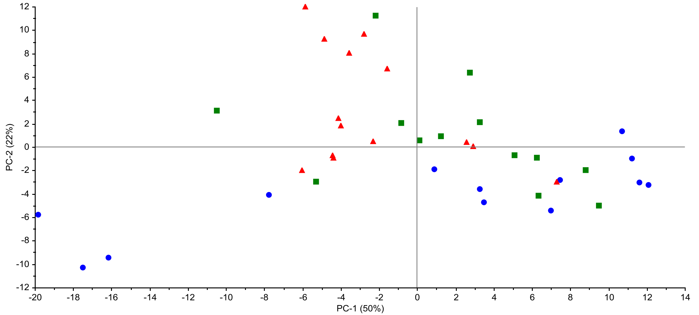
Scores
